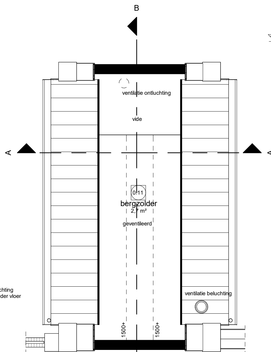
Bergzolder
