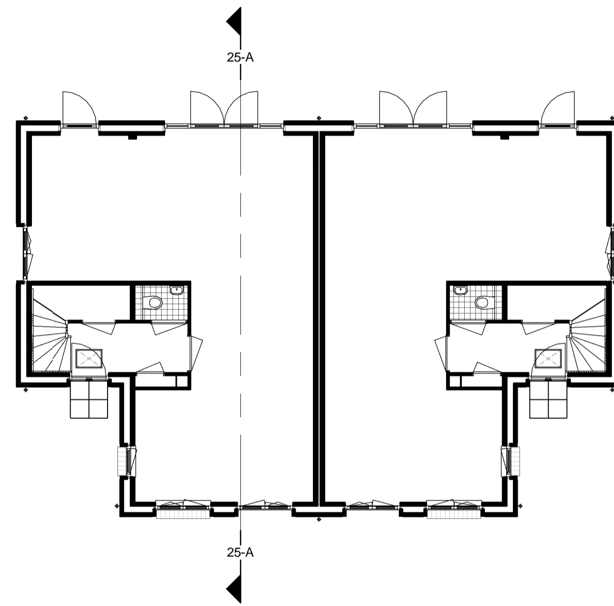
Begane grond Type H3 bwnr. 169 Type H3s bwnr. 170
